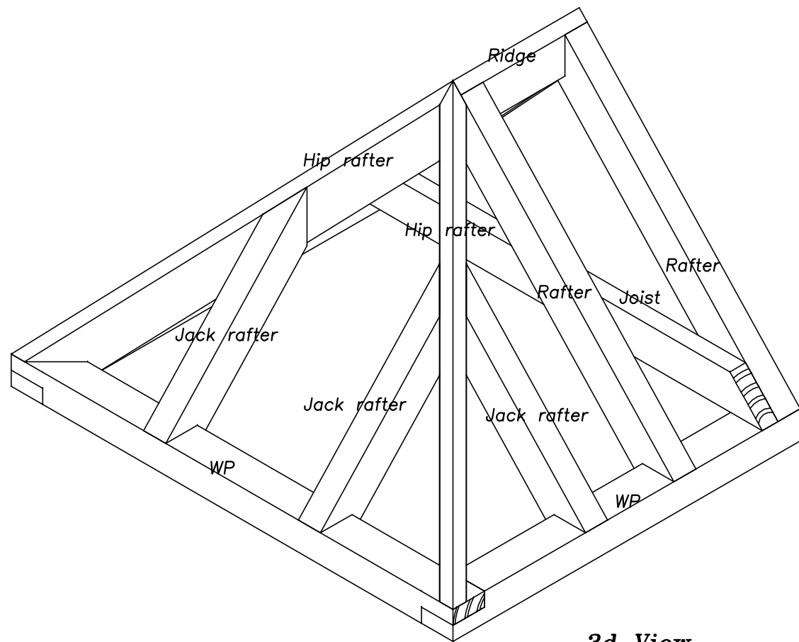
3d View
