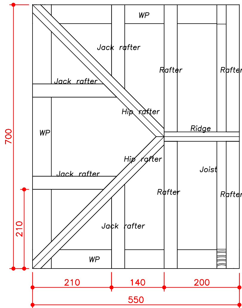
Plan
