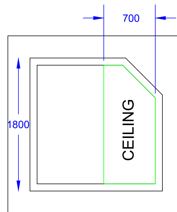
ELEVATION D
