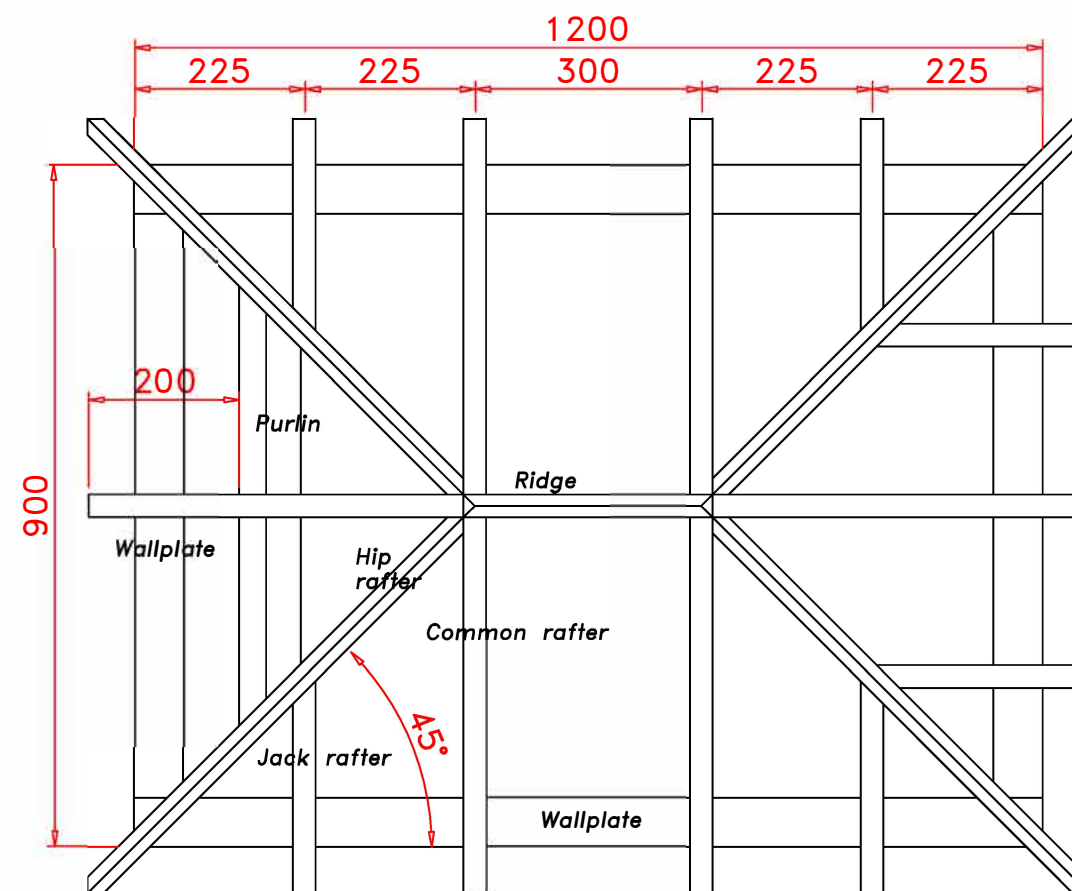
PLAN
