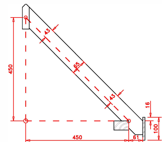
Common rafter dimensions
