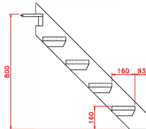
Steps detail
