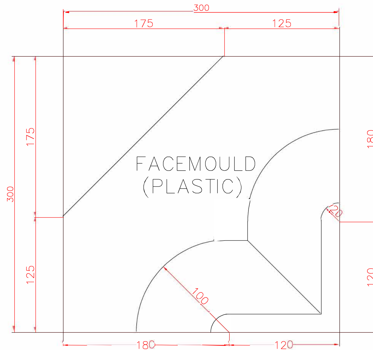
PLAN VIEW
