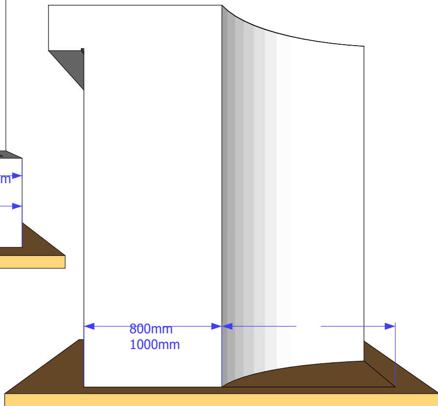
Elevation D
