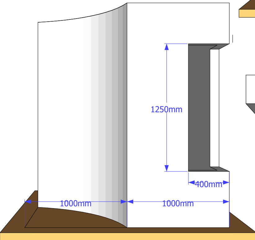
Elevation C
