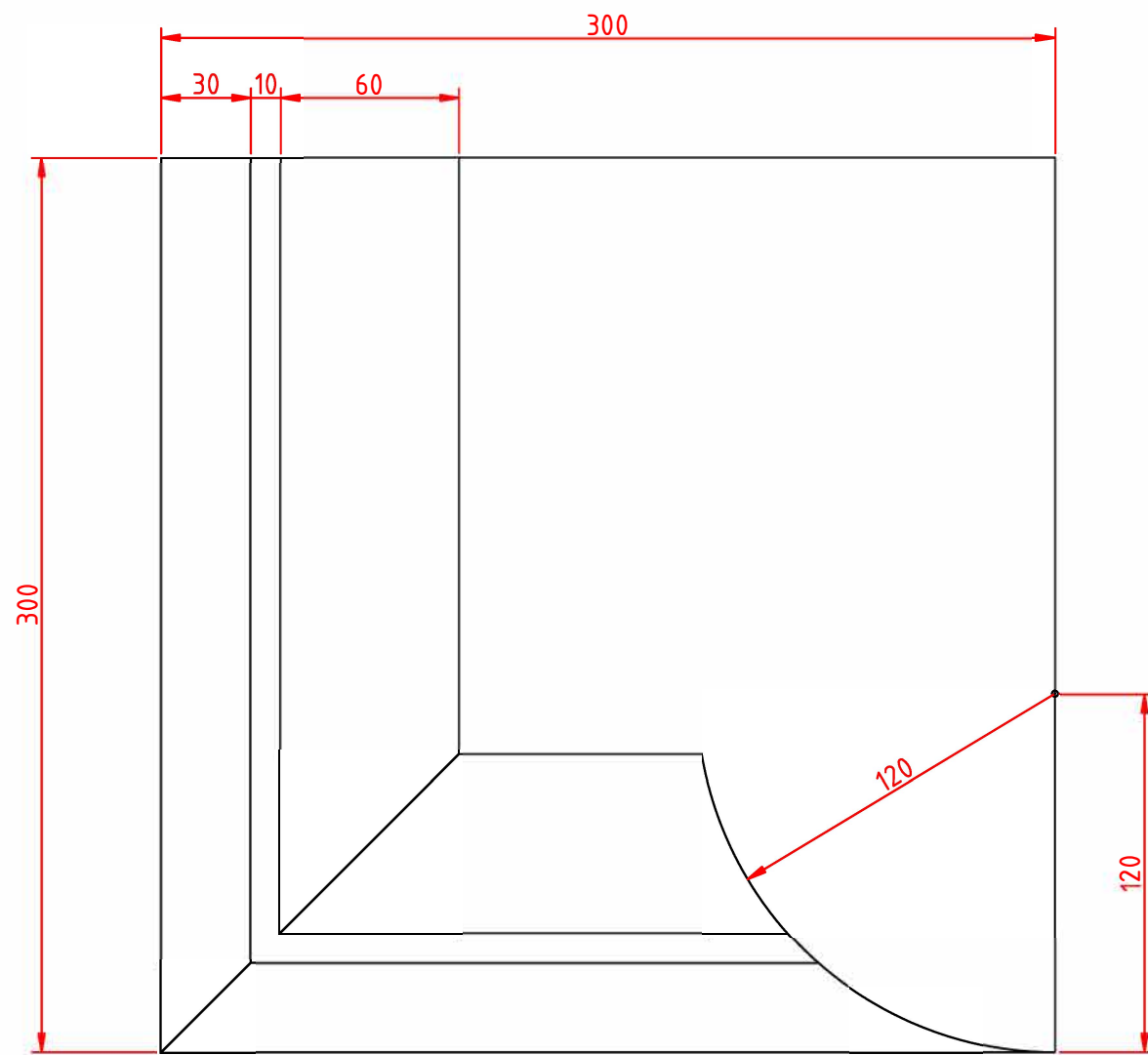
Plan View
